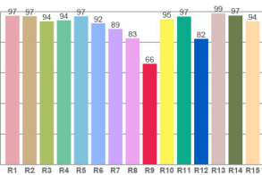
CRI: 92.8 (R1-R8)
